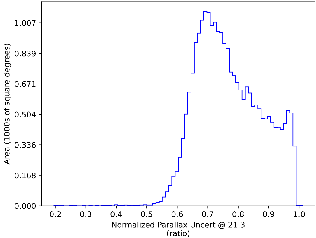
too_elab_r8_d2_ugrizy_v3.4_10yrs All sky y band only: Normalized Parallax Uncert @ 21.3
