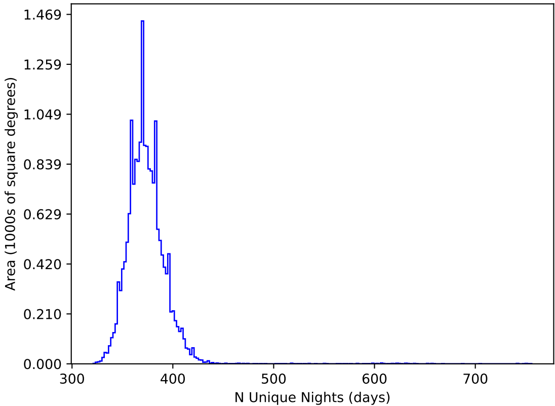
too_elab_r8_d2_ugrizy_v3.4_10yrs WFD all bands: N Unique Nights
