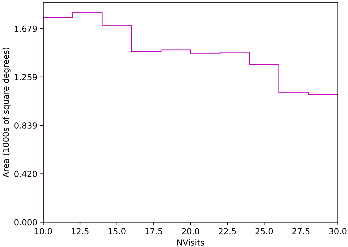
too_elab_r8_d2_ugrizy_v3.4_10yrs Yr 3-4 z band: NVisits
