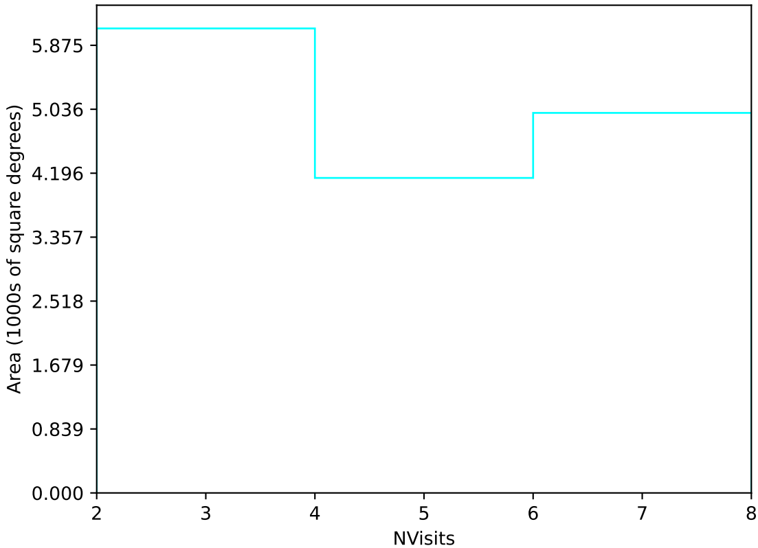
too_elab_r8_d2_ugrizy_v3.4_10yrs Yr 3-4 u band: NVisits
