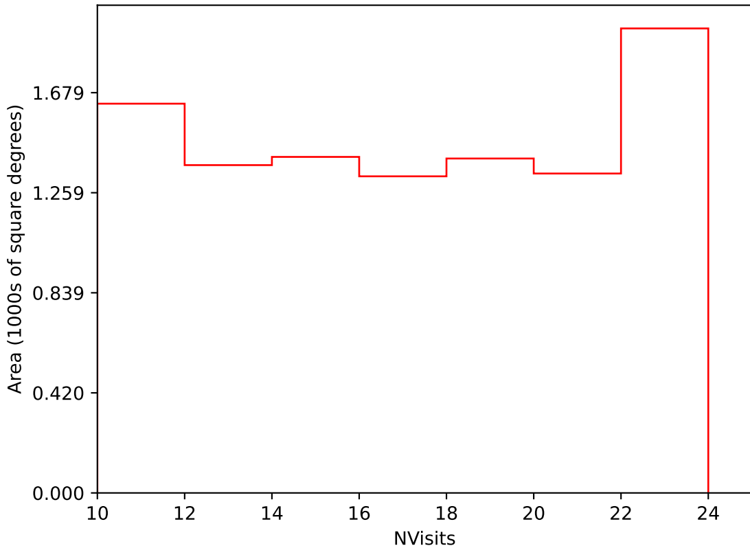
too_elab_r8_d2_ugrizy_v3.4_10yrs Yr 3-4 i band: NVisits
