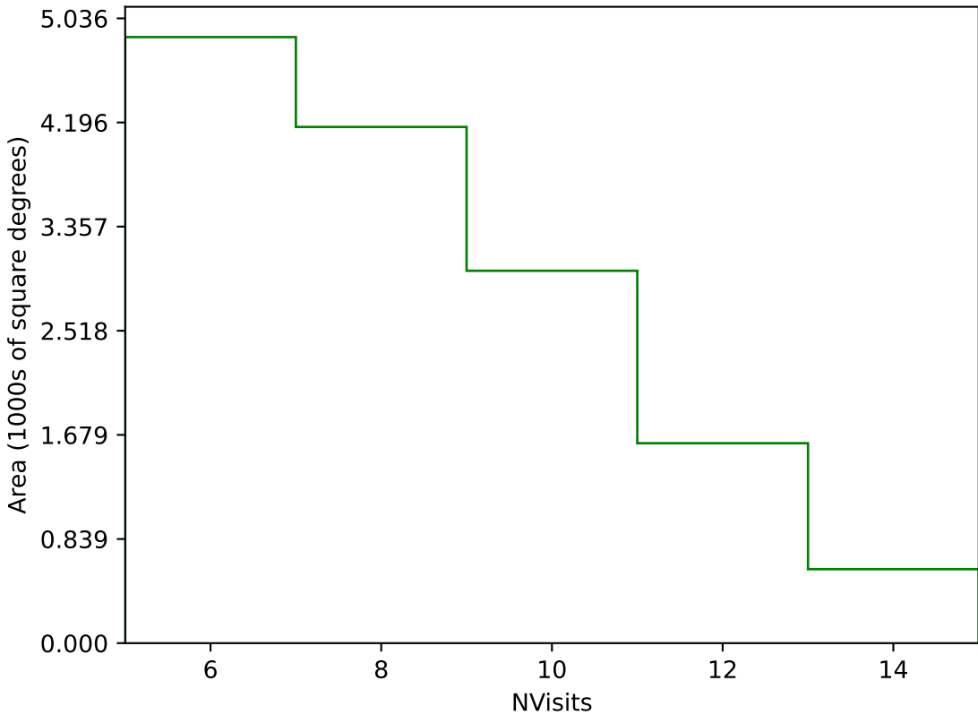
too_elab_r8_d2_ugrizy_v3.4_10yrs Yr 3-4 g band: NVisits
