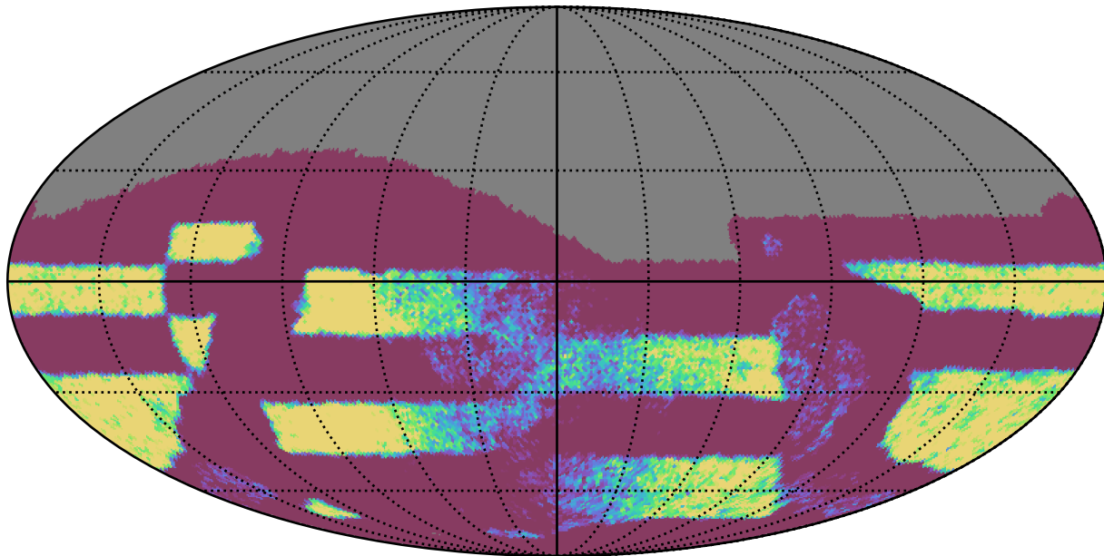
too_elab_r8_d2_ugrizy_v3.4_10yrs Yr 3-4 all bands: NVisits
