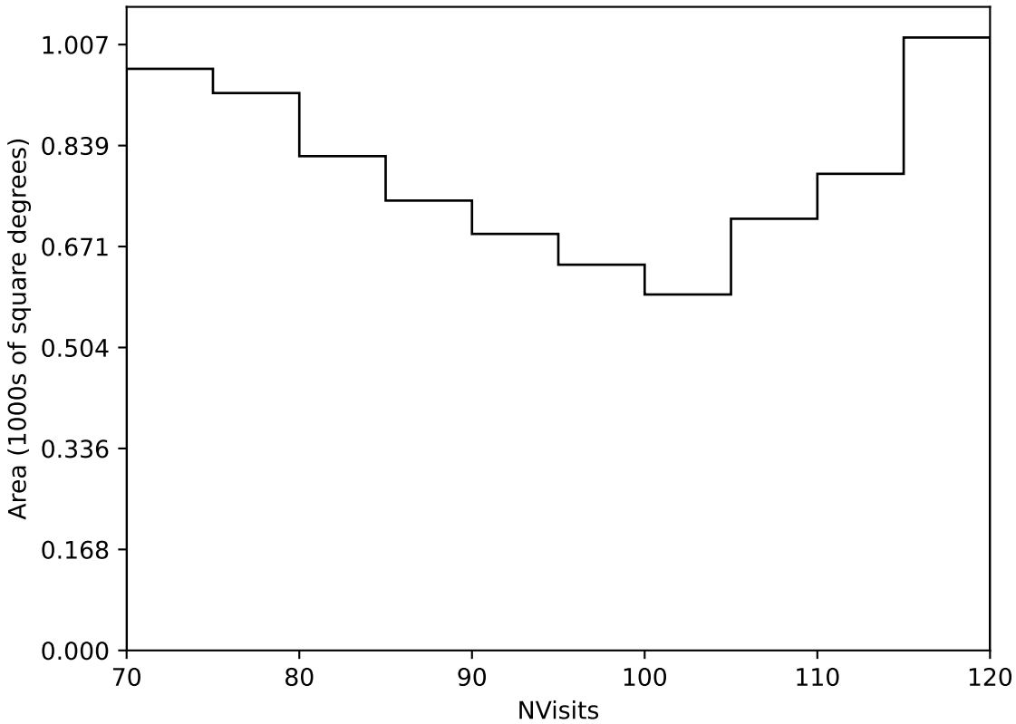
too_elab_r8_d2_ugrizy_v3.4_10yrs Yr 3-4 all bands: NVisits
