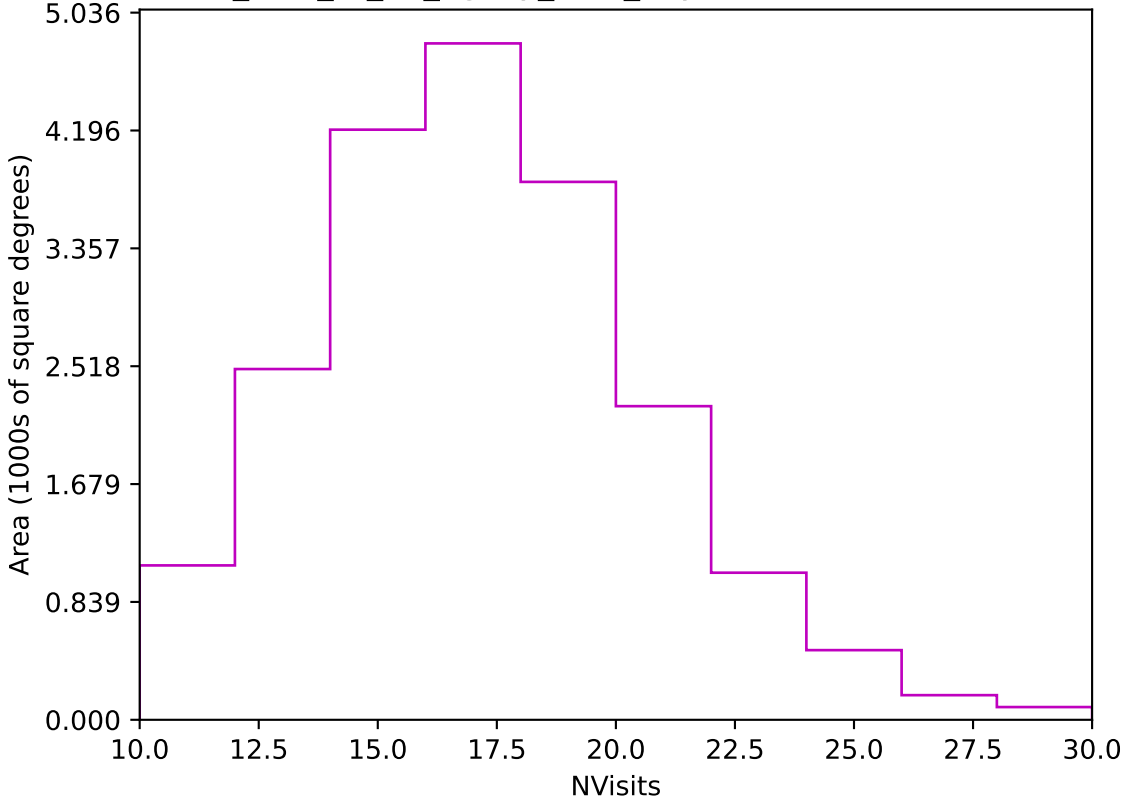
too_elab_r8_d2_ugrizy_v3.4_10yrs Yr 1 z band: NVisits
