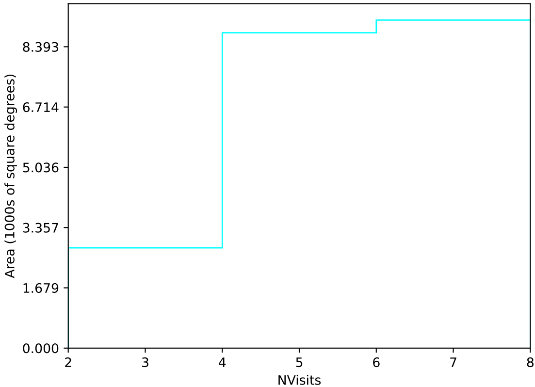
too_elab_r8_d2_ugrizy_v3.4_10yrs Yr 1 u band: NVisits
