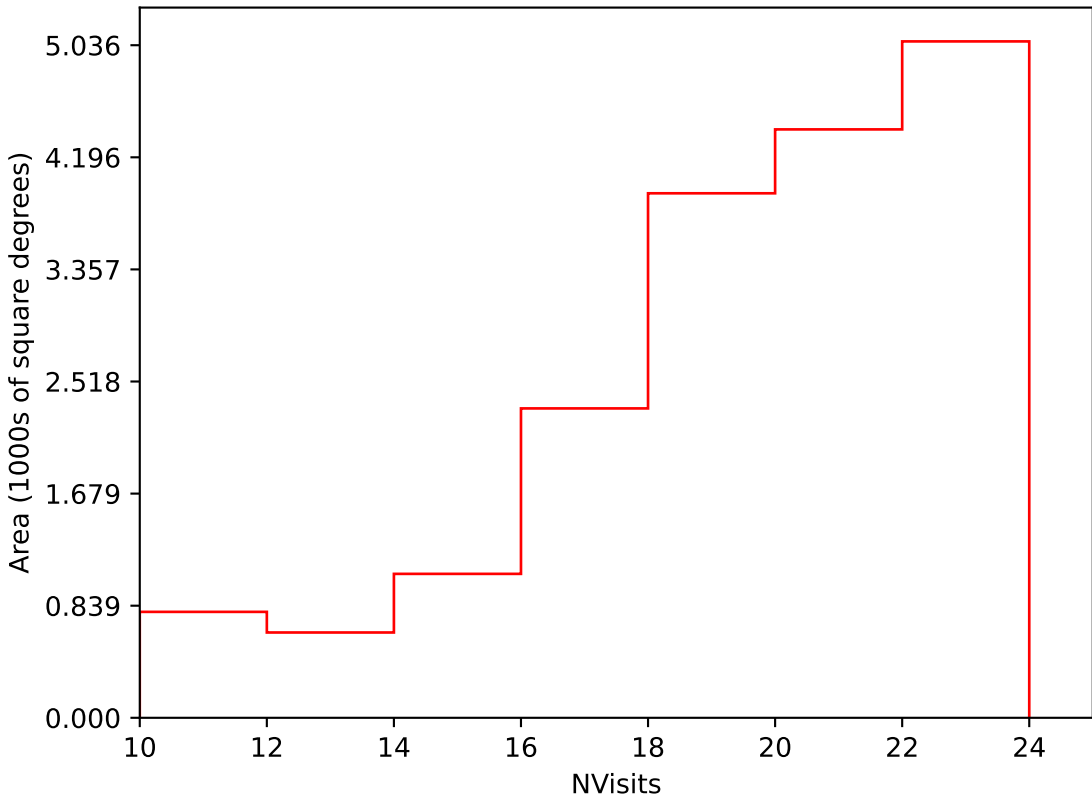
too_elab_r8_d2_ugrizy_v3.4_10yrs Yr 1 i band: NVisits
