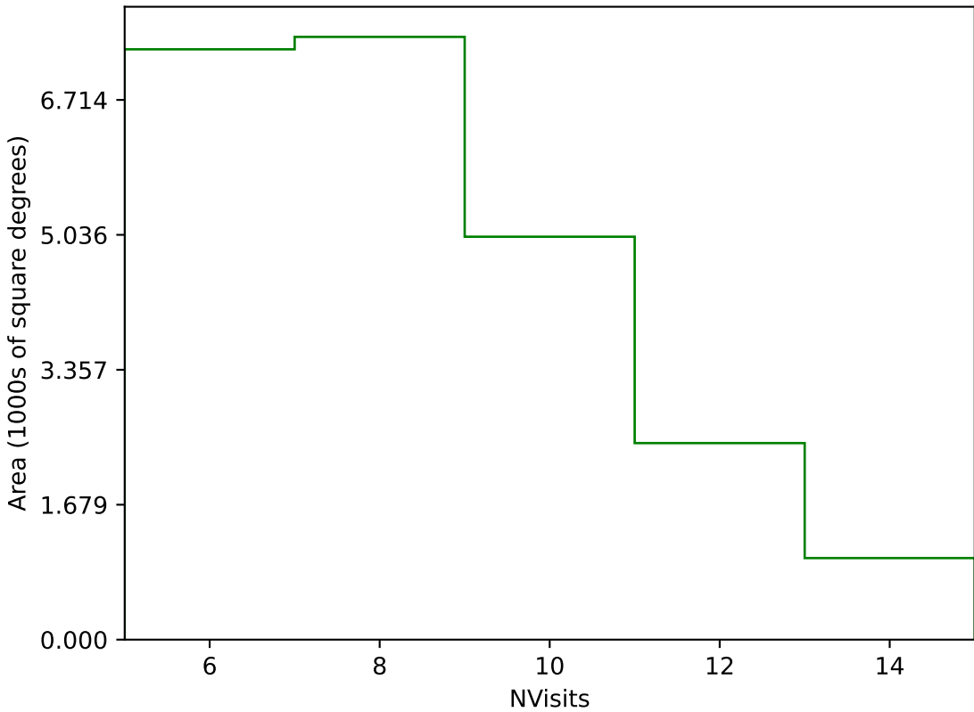
too_elab_r8_d2_ugrizy_v3.4_10yrs Yr 1 g band: NVisits
