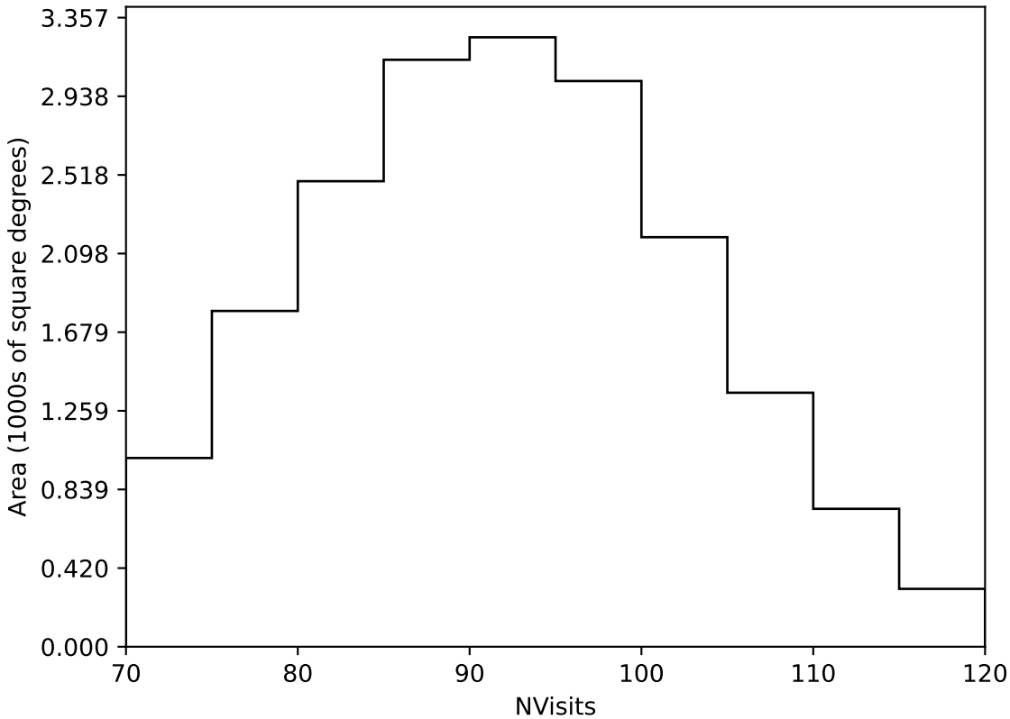
too_elab_r8_d2_ugrizy_v3.4_10yrs Yr 1 all bands: NVisits
