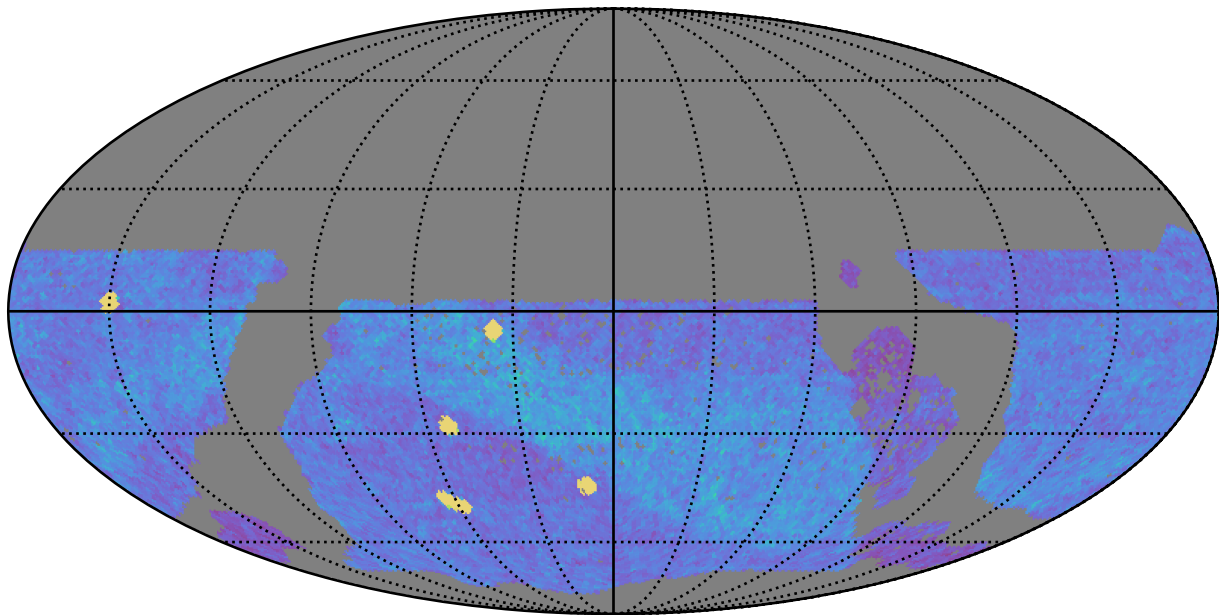
too_elab_r8_d2_ugrizy_v3.4_10yrs WFD z band: NVisits
