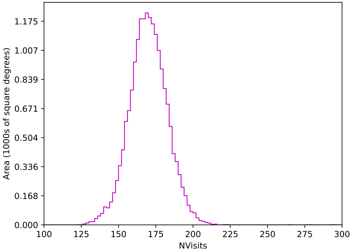
too_elab_r8_d2_ugrizy_v3.4_10yrs WFD z band: NVisits
