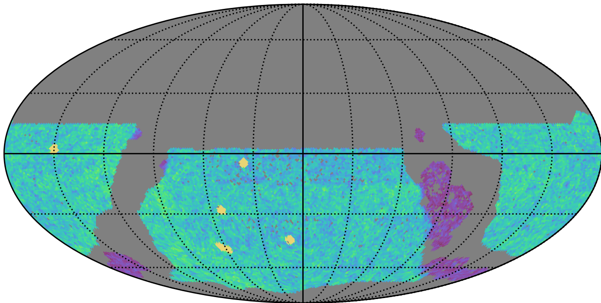
too_elab_r8_d2_ugrizy_v3.4_10yrs WFD u band: NVisits
