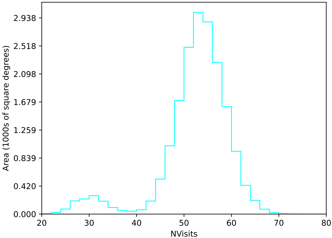
too_elab_r8_d2_ugrizy_v3.4_10yrs WFD u band: NVisits
