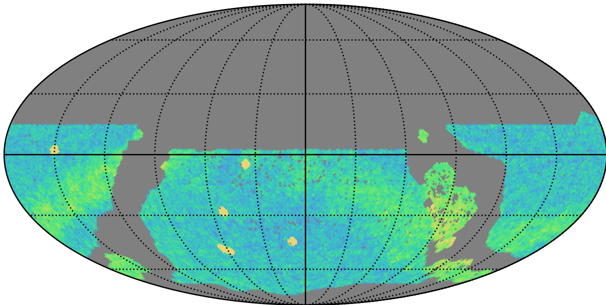
too_elab_r8_d2_ugrizy_v3.4_10yrs WFD r band: NVisits
