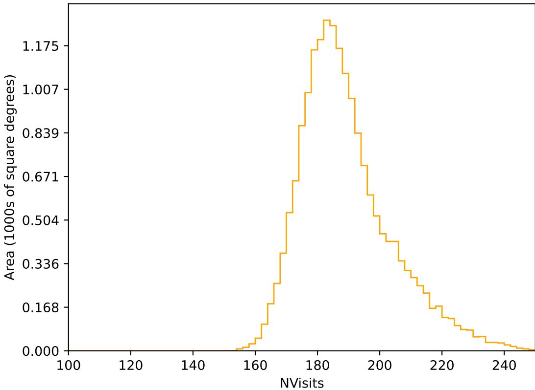
too_elab_r8_d2_ugrizy_v3.4_10yrs WFD r band: NVisits
