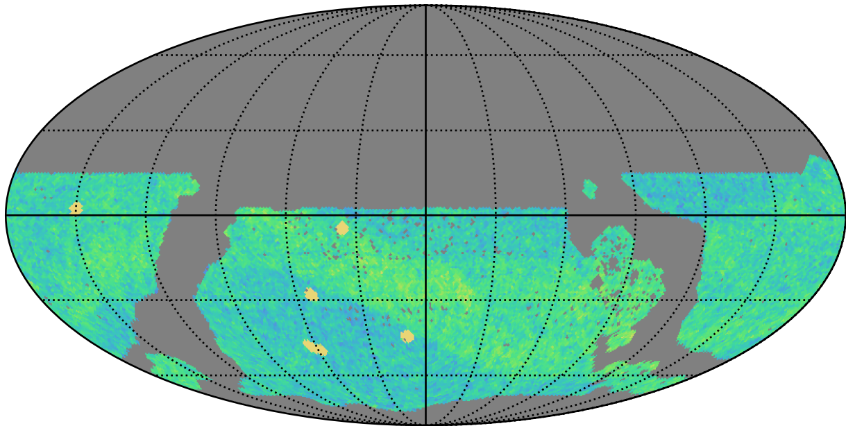
too_elab_r8_d2_ugrizy_v3.4_10yrs WFD i band: NVisits
