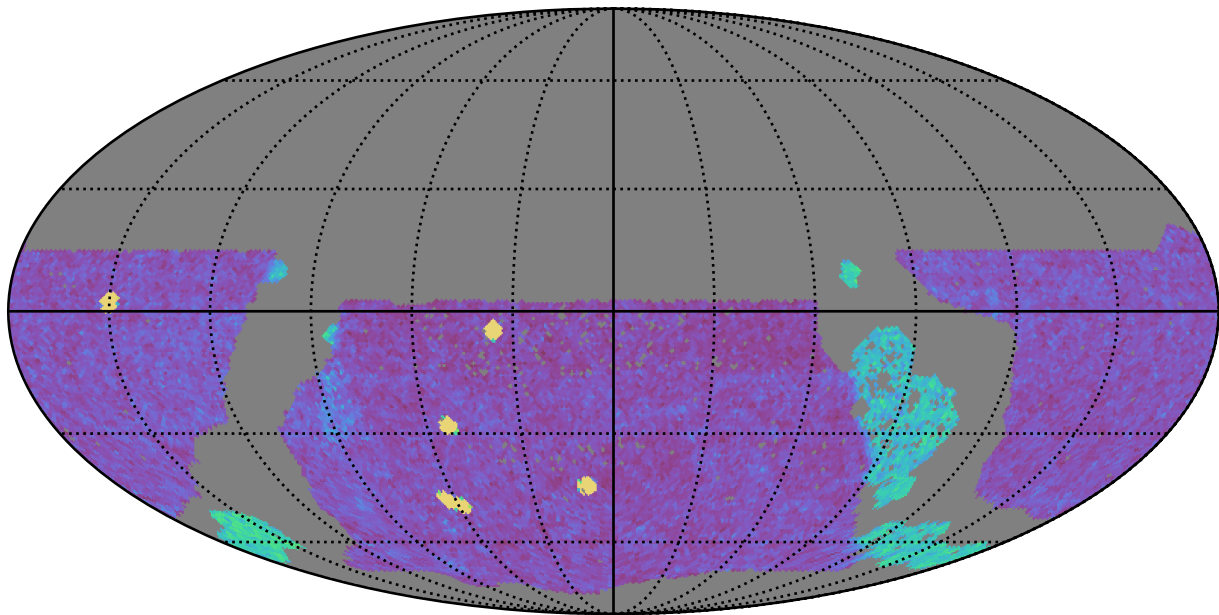
too_elab_r8_d2_ugrizy_v3.4_10yrs WFD g band: NVisits
