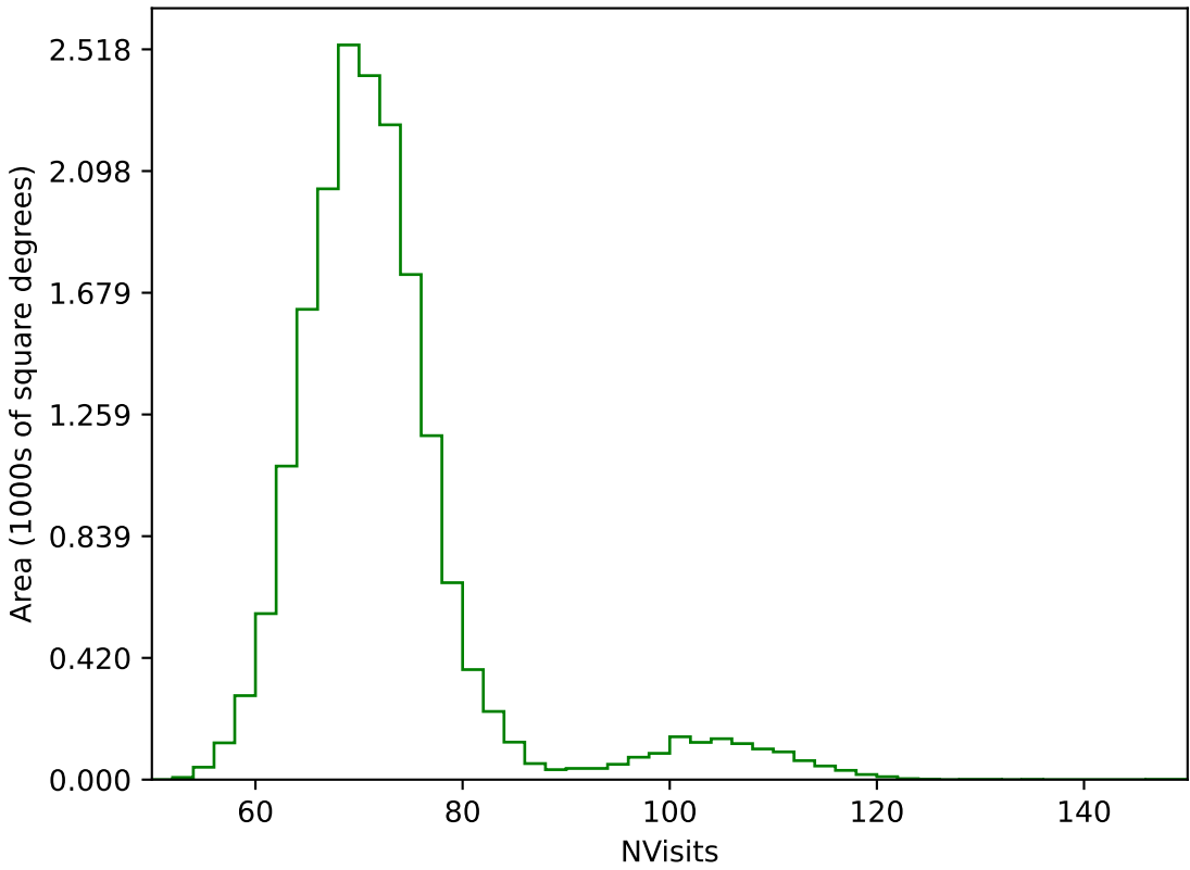
too_elab_r8_d2_ugrizy_v3.4_10yrs WFD g band: NVisits
