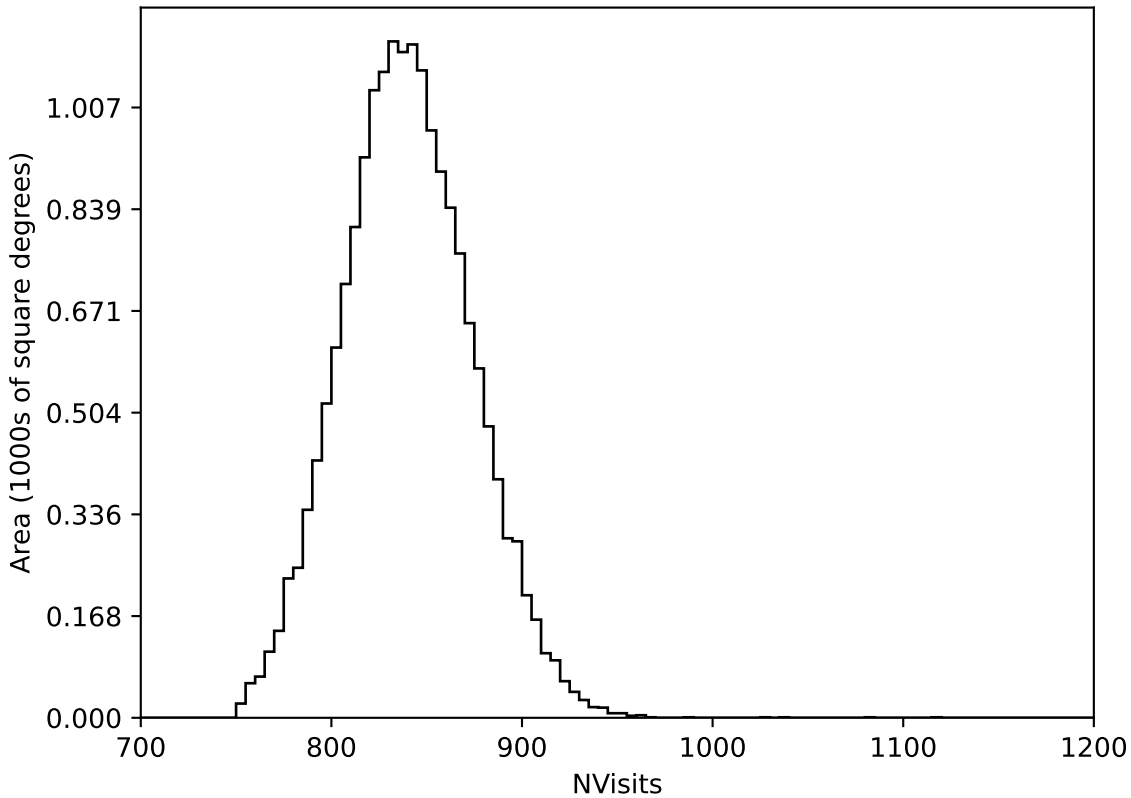
too_elab_r8_d2_ugrizy_v3.4_10yrs WFD all bands: NVisits
