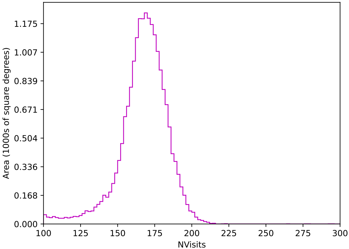
too_elab_r8_d2_ugrizy_v3.4_10yrs All sky z band: NVisits
