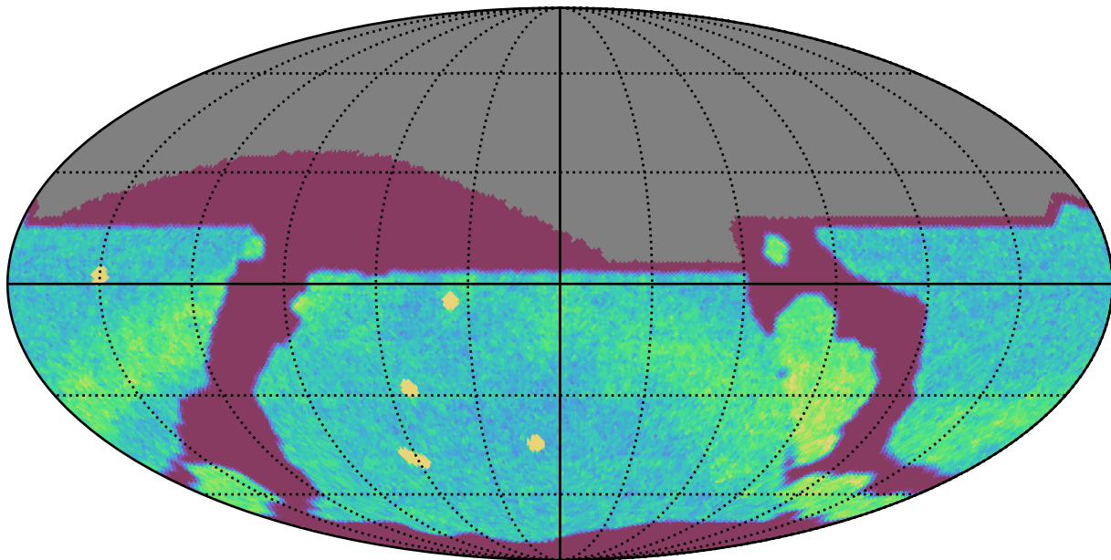
too_elab_r8_d2_ugrizy_v3.4_10yrs All sky r band: NVisits
