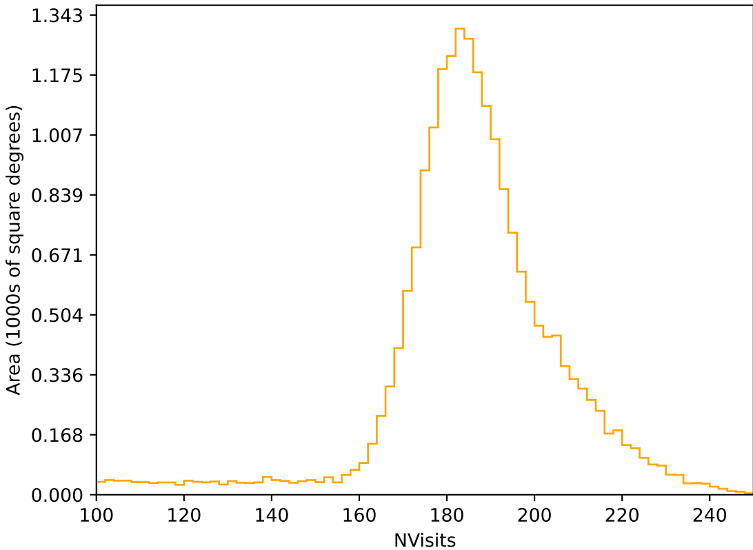
too_elab_r8_d2_ugrizy_v3.4_10yrs All sky r band: NVisits
