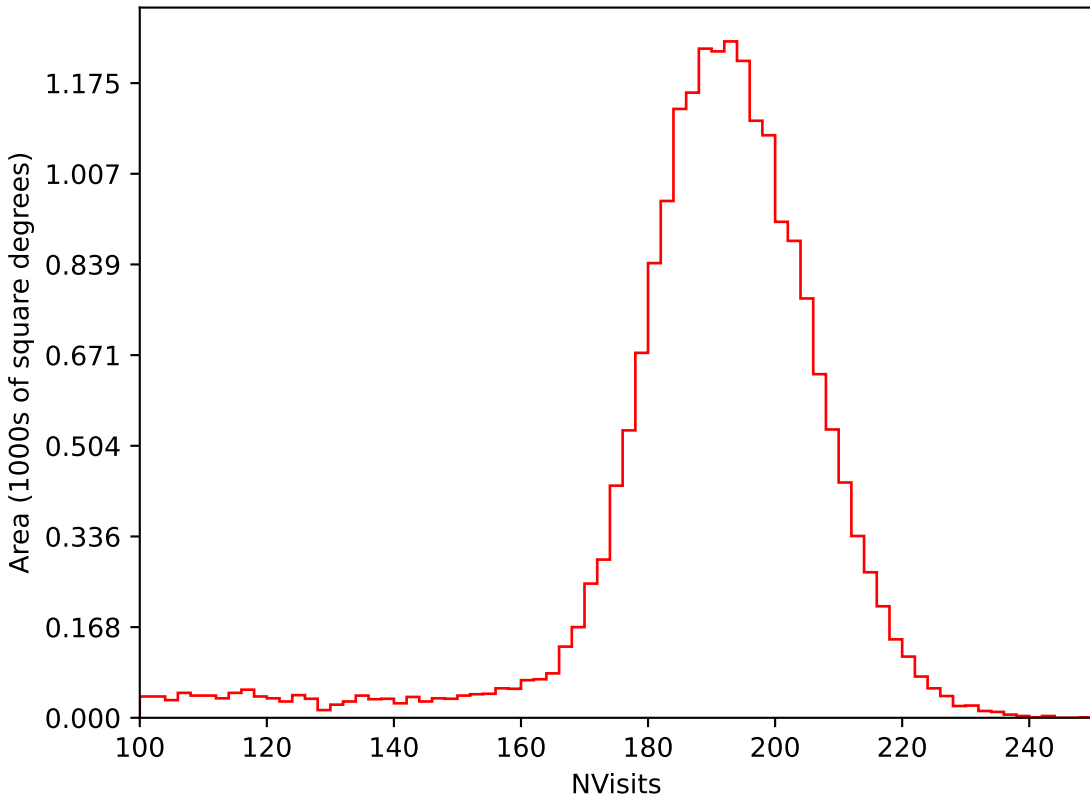
too_elab_r8_d2_ugrizy_v3.4_10yrs All sky i band: NVisits
