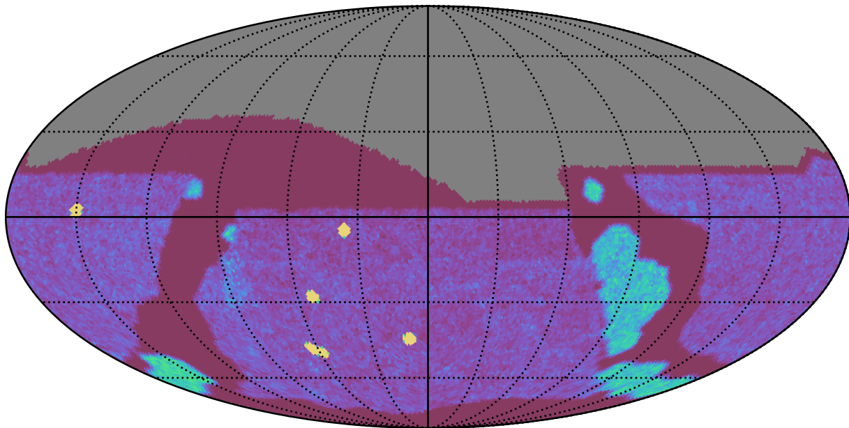
too_elab_r8_d2_ugrizy_v3.4_10yrs All sky g band: NVisits
