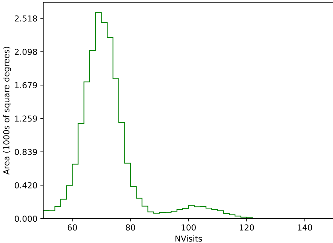
too_elab_r8_d2_ugrizy_v3.4_10yrs All sky g band: NVisits
