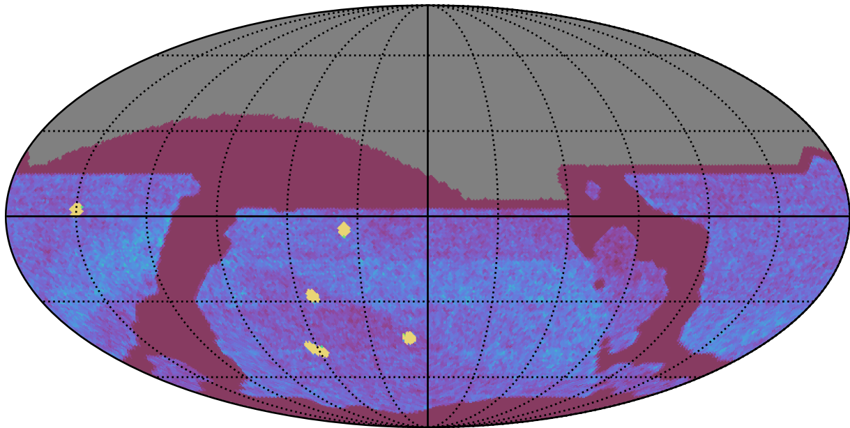
too_elab_r8_d2_ugrizy_v3.4_10yrs All sky all bands: NVisits
