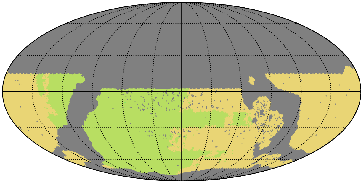
too_elab_r8_d2_ugrizy_v3.4_10yrs WFD all bands: NSeasons
