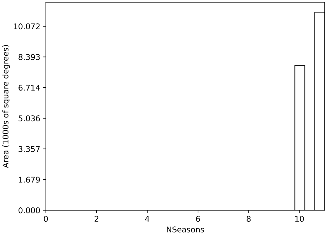
too_elab_r8_d2_ugrizy_v3.4_10yrs WFD all bands: NSeasons
