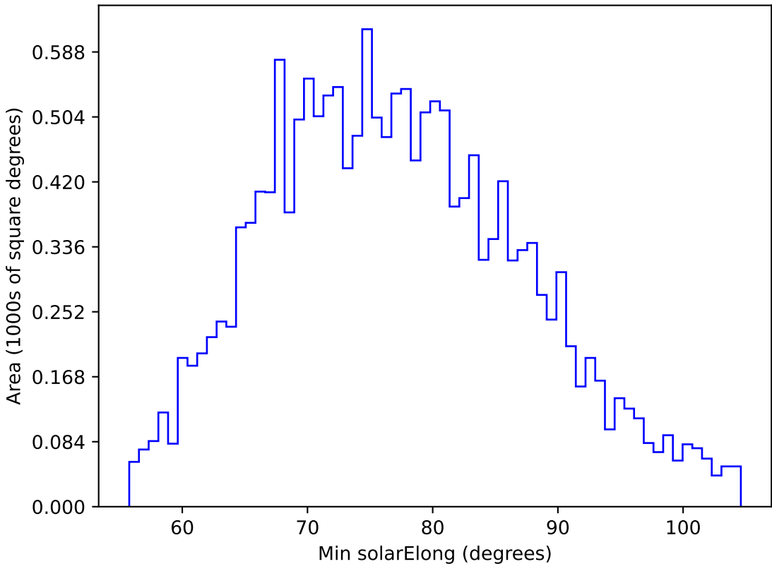
too_elab_r8_d2_ugrizy_v3.4_10yrs WFD u band: Min solarElong
