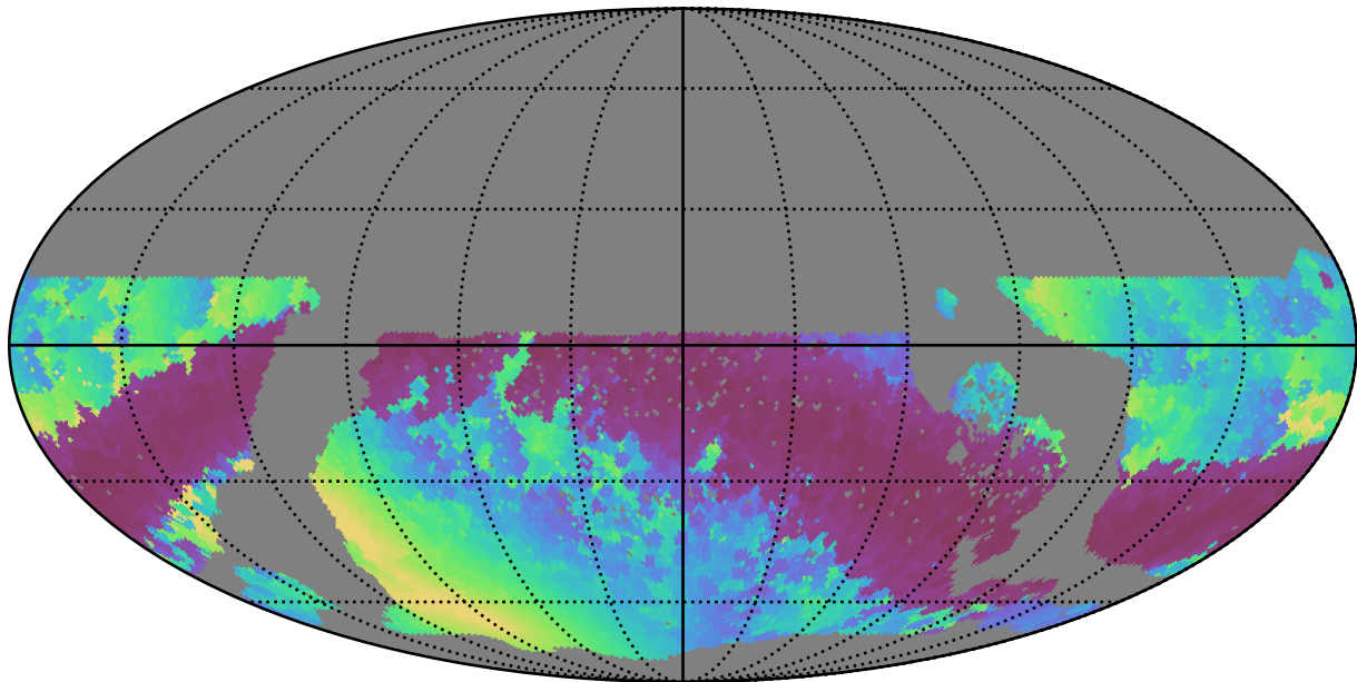
too_elab_r8_d2_ugrizy_v3.4_10yrs WFD r band: Min solarElong
