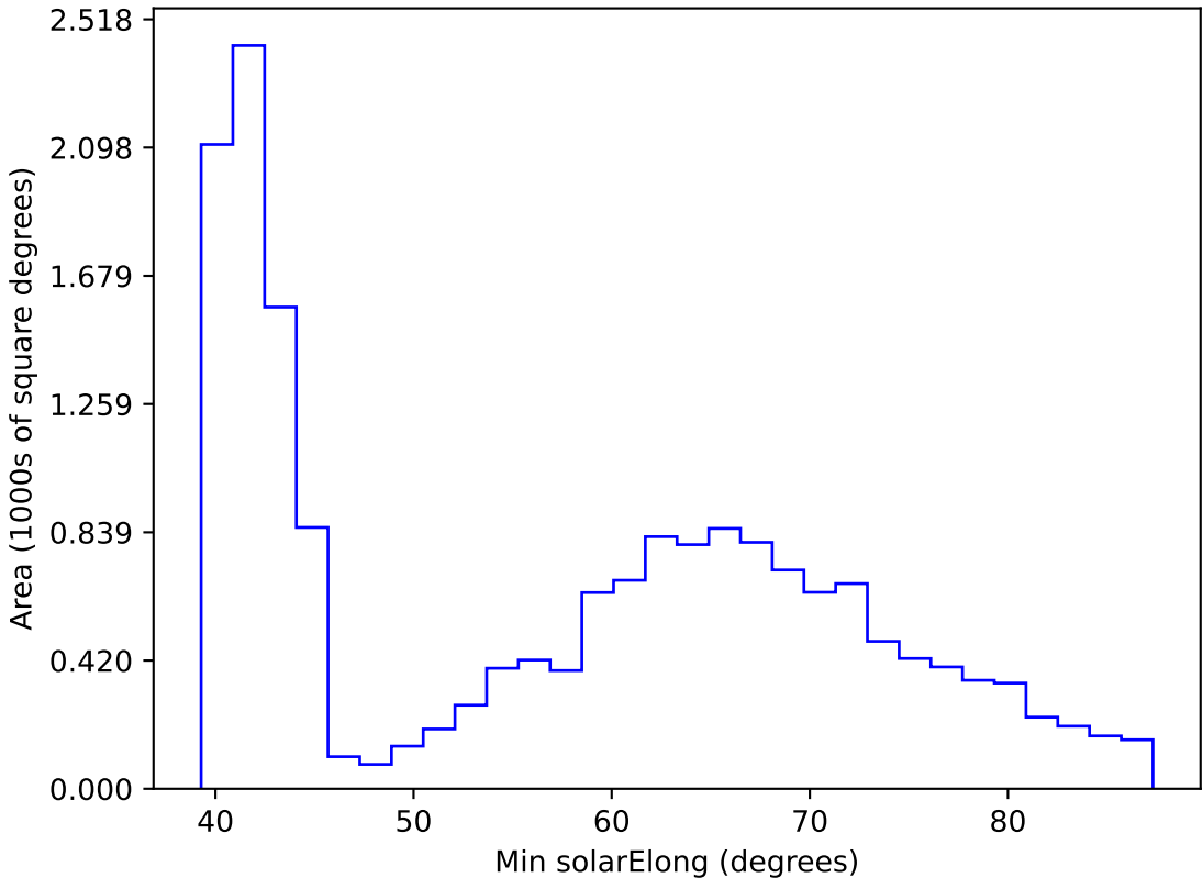
too_elab_r8_d2_ugrizy_v3.4_10yrs WFD r band: Min solarElong
