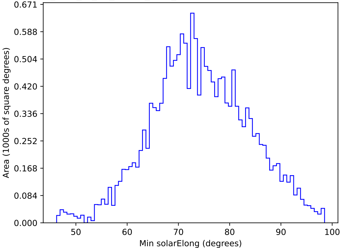
too_elab_r8_d2_ugrizy_v3.4_10yrs WFD g band: Min solarElong
