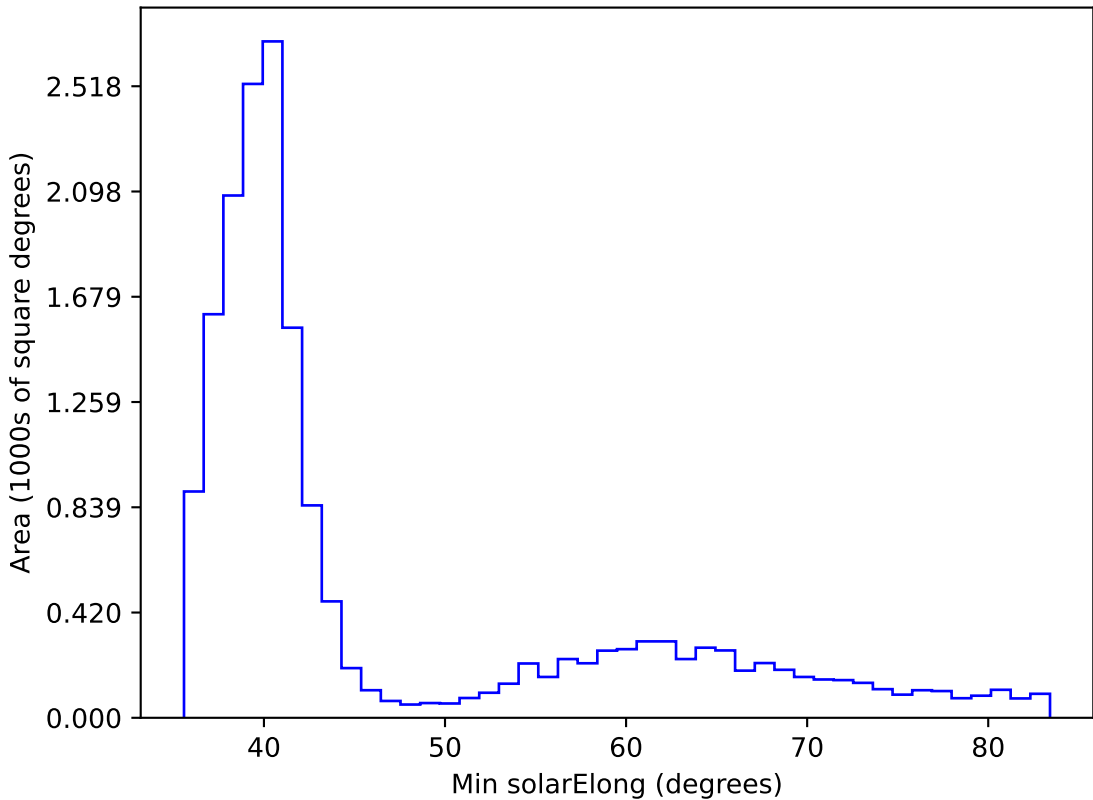
too_elab_r8_d2_ugrizy_v3.4_10yrs WFD all bands: Min solarElong
