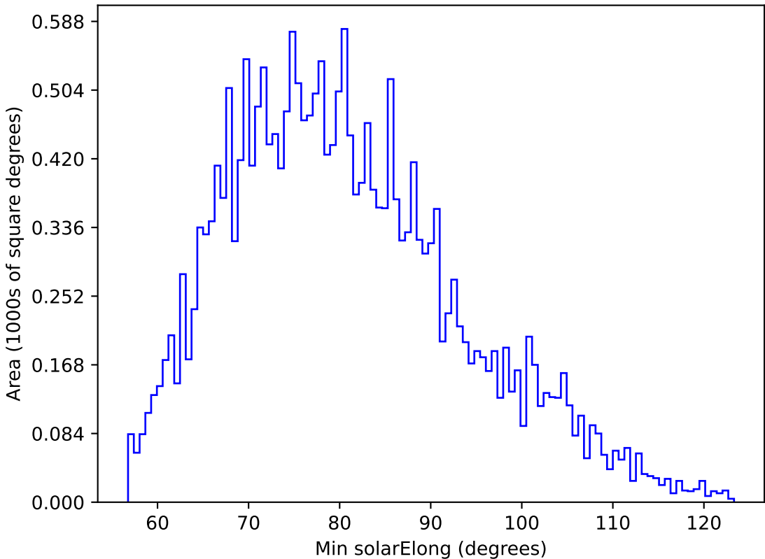
too_elab_r8_d2_ugrizy_v3.4_10yrs All sky u band: Min solarElong
