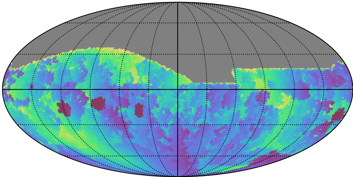
too_elab_r8_d2_ugrizy_v3.4_10yrs All sky g band: Min solarElong
