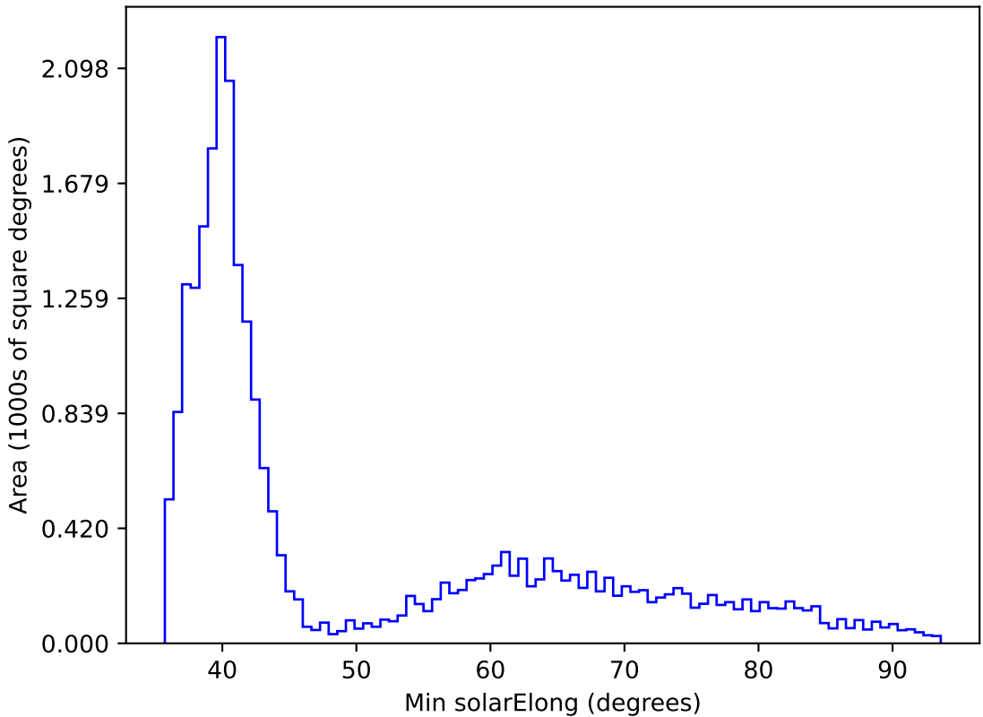
too_elab_r8_d2_ugrizy_v3.4_10yrs All sky all bands: Min solarElong
