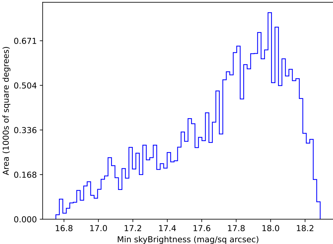
too_elab_r8_d2_ugrizy_v3.4_10yrs Yr 1 y band: Min skyBrightness
