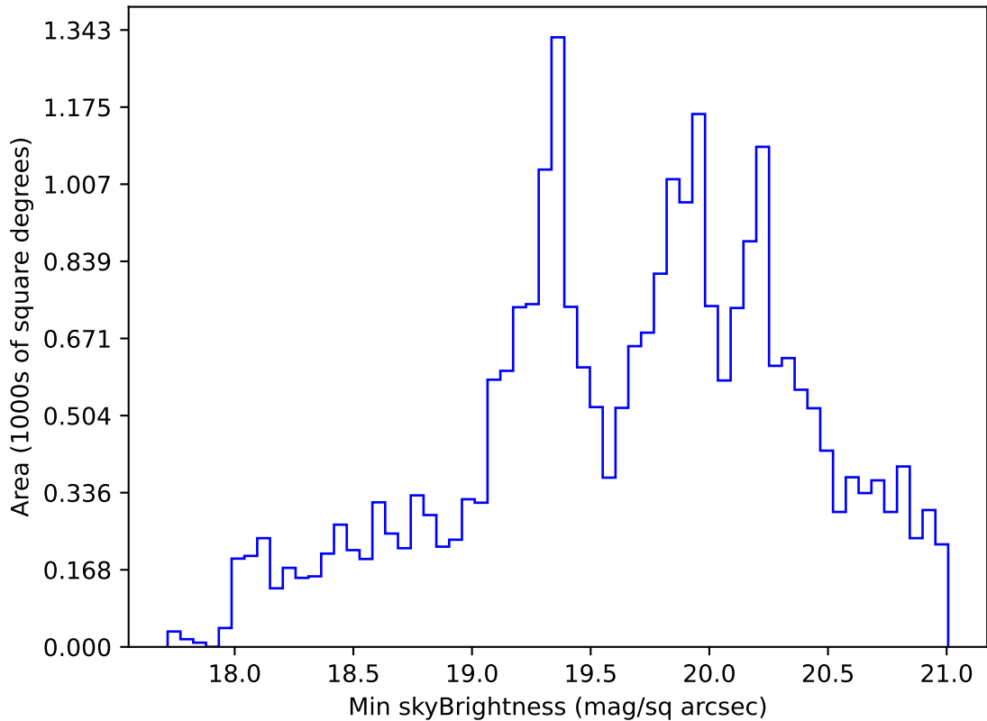
too_elab_r8_d2_ugrizy_v3.4_10yrs Yr 1 r band: Min skyBrightness
