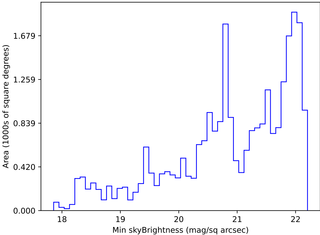
too_elab_r8_d2_ugrizy_v3.4_10yrs Yr 1 g band: Min skyBrightness
