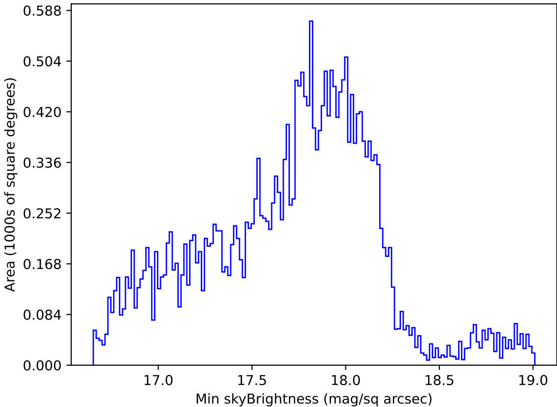
too_elab_r8_d2_ugrizy_v3.4_10yrs Yr 1 all bands: Min skyBrightness
