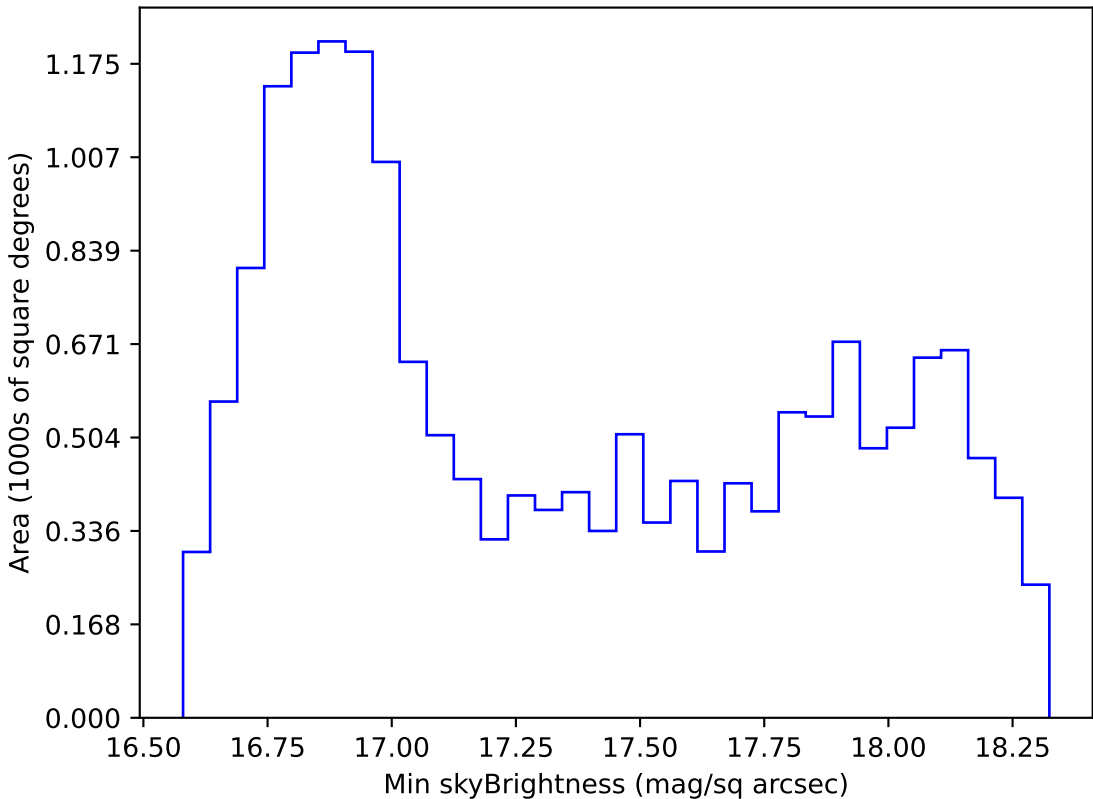
too_elab_r8_d2_ugrizy_v3.4_10yrs WFD z band: Min skyBrightness
