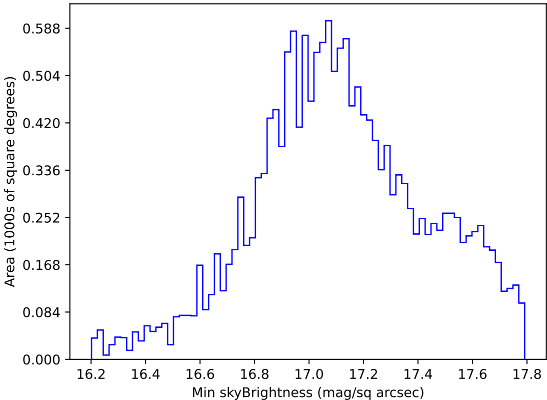
too_elab_r8_d2_ugrizy_v3.4_10yrs WFD y band: Min skyBrightness
