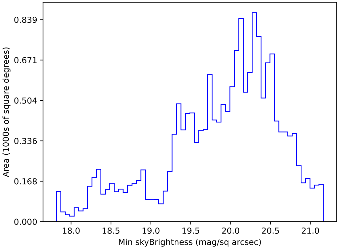
too_elab_r8_d2_ugrizy_v3.4_10yrs WFD g band: Min skyBrightness
