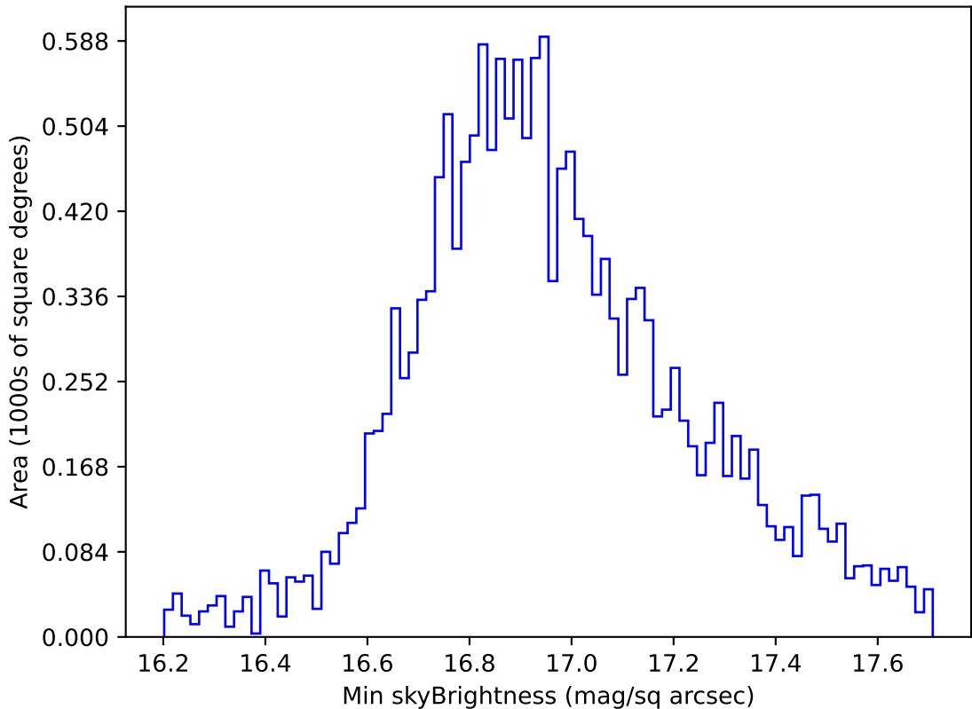
too_elab_r8_d2_ugrizy_v3.4_10yrs WFD all bands: Min skyBrightness
