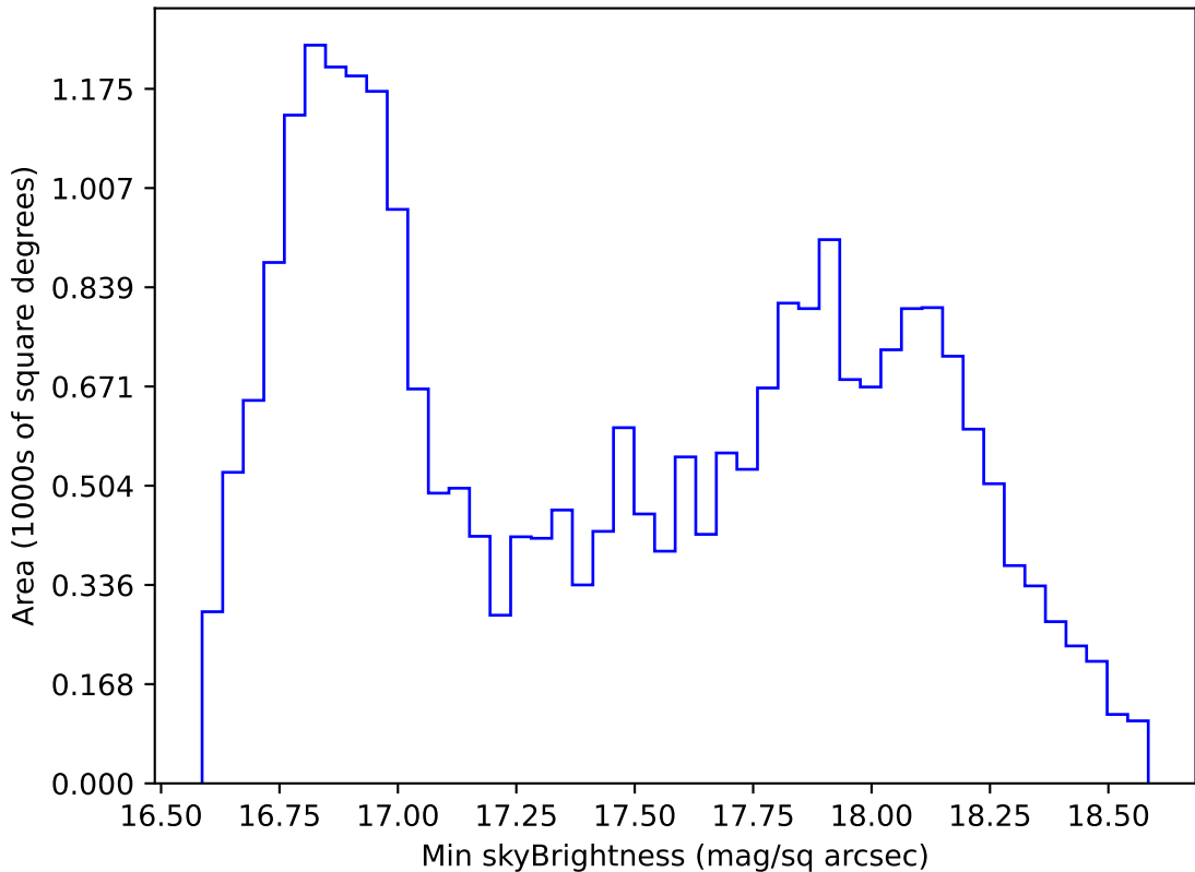
too_elab_r8_d2_ugrizy_v3.4_10yrs All sky z band: Min skyBrightness
