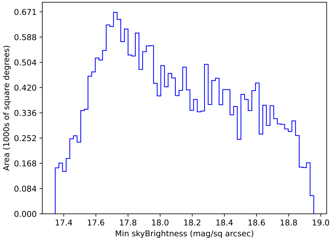
too_elab_r8_d2_ugrizy_v3.4_10yrs All sky i band: Min skyBrightness
